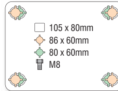
100mm swivel
