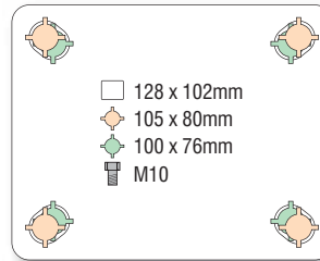
100mm swivel
