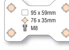
75mm fixed
