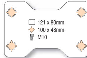
100mm fixed
