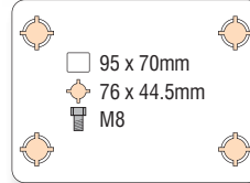
75mm swivel
