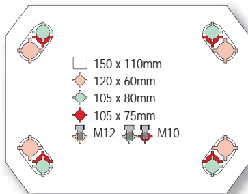
2SH (swivel)
