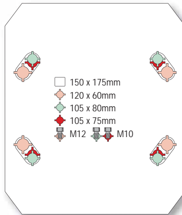
2FH (fixed)
